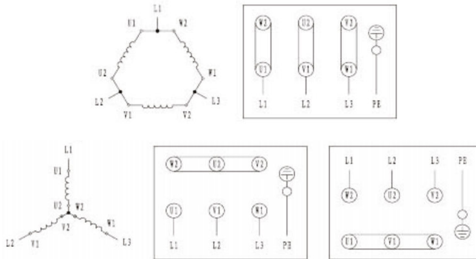
Figure 1 - Connection Diagram
