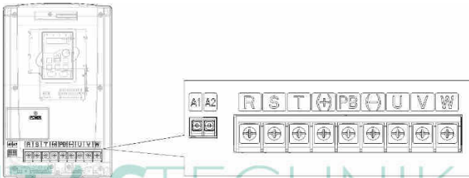
Fig 4-12 22~30kW
