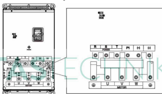
Fig 4-15 132~200kW
